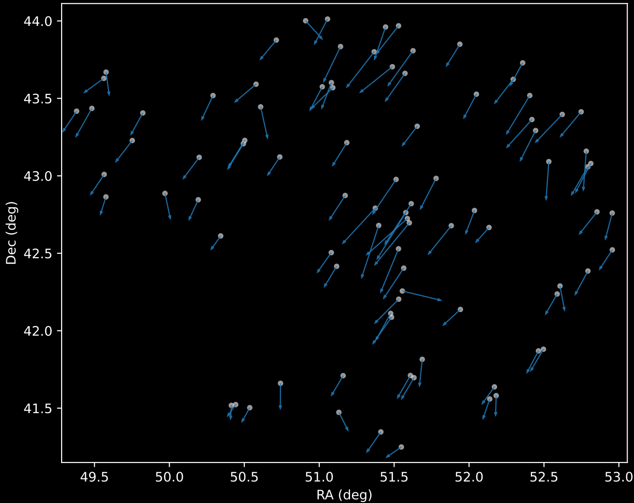
APOGEE DR17 Cluster 0 Proper Motion Vectors (n=89)
